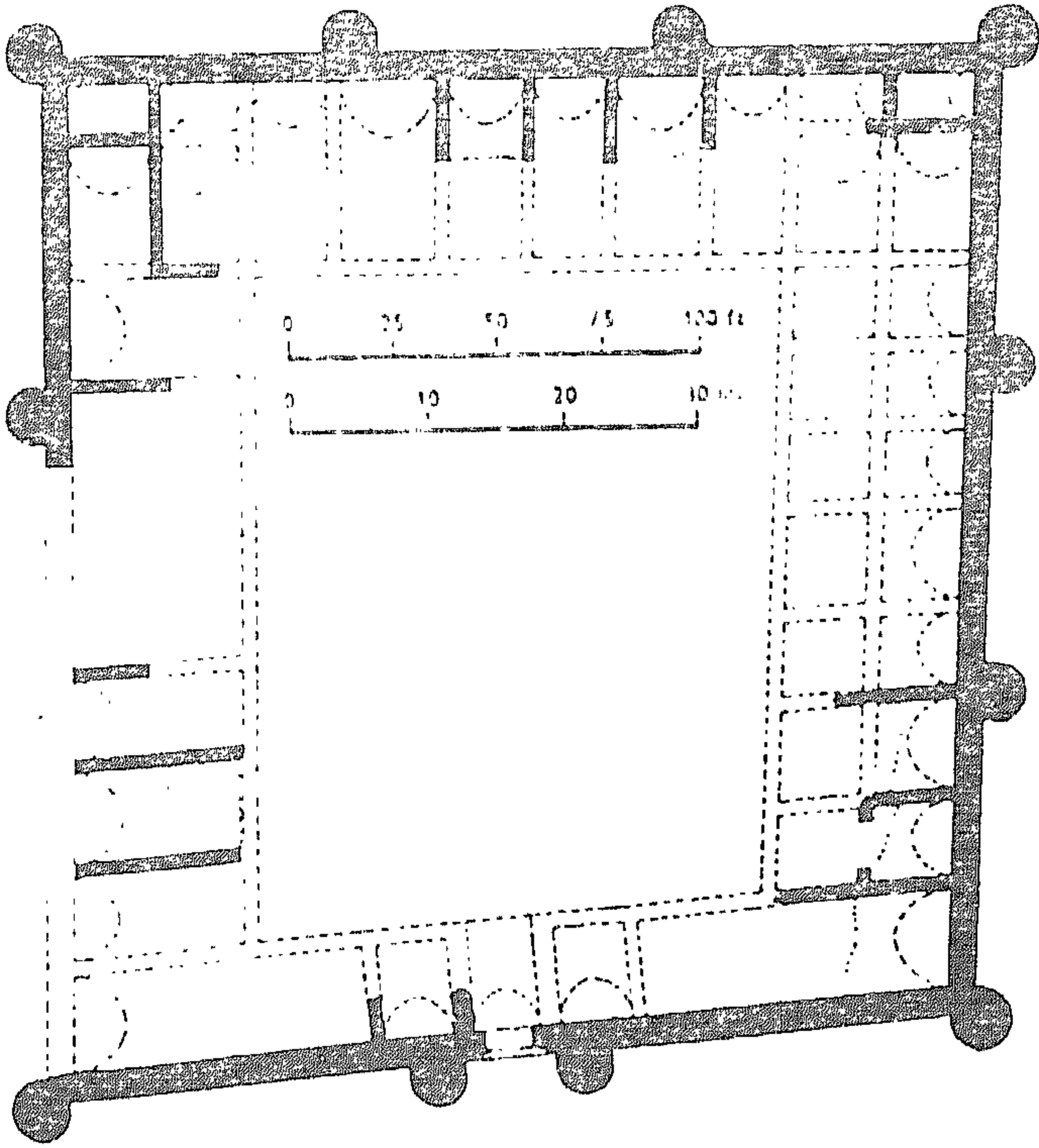
Figure 19. Qasr al-Hair: plan of Letter Enclosure
